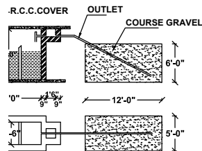
ANK & D-TRENCH DETAILS (NOT TO SCALE)
