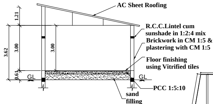
SECTION X - X
