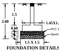
FOUNDATION DETAILS
