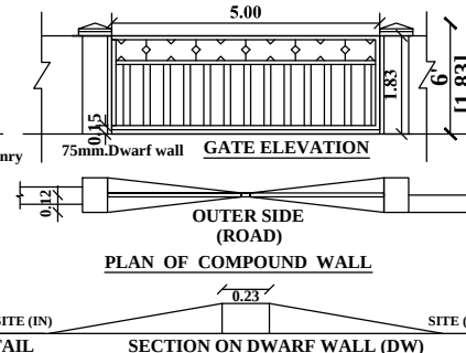
SECTION ON DWARF WALL (DW)
