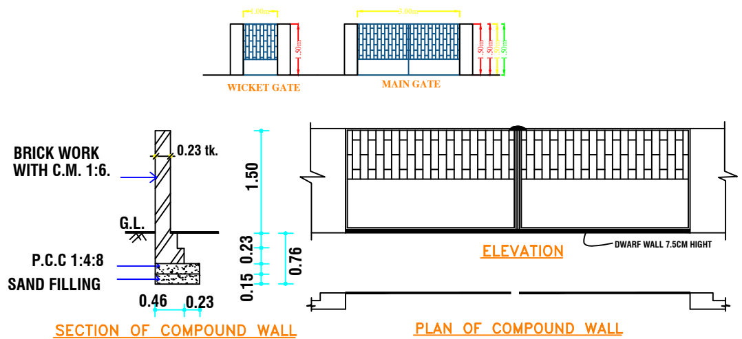
COMPOUND WALL
