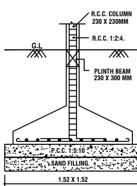
FOUNDATION DETAIL
