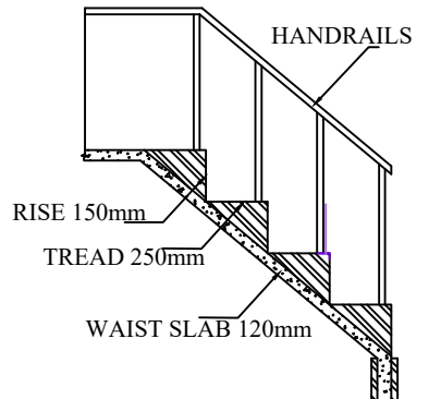
STAIRCASE DETAILS
