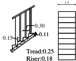
STAIRCASE DETAIL
