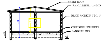
CUT SECTION ON AA
