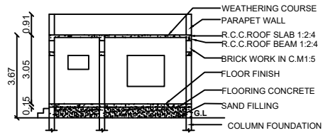
SECTION ON SS
