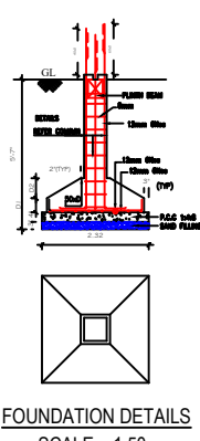
FOUNDATION DETAILS SCALE : 1:50.
