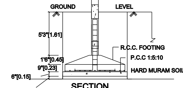
FOUNDATION DETAILS
