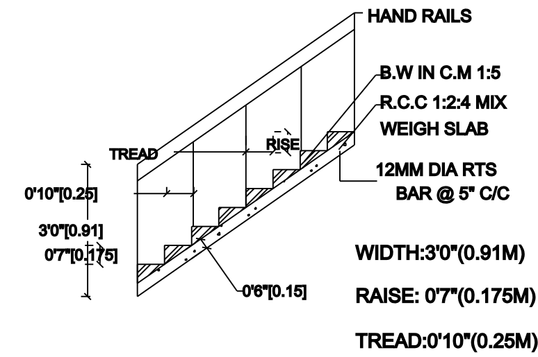
STAIR CASE DETAILS:-
