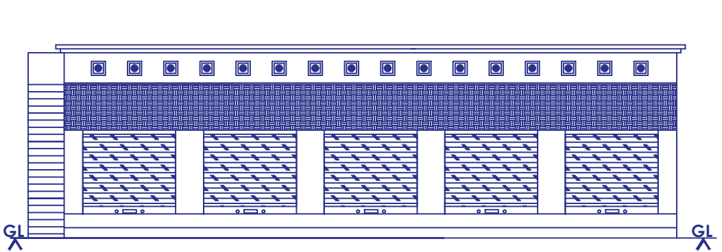
FRONT ELEVATION
