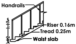
STAIRCASE DETAILS FLR_HT_M=3.05 FLR_HT_M=03.05
