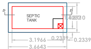
PLAN OF SEPTIC TANK SCALE 1"=2'0"
