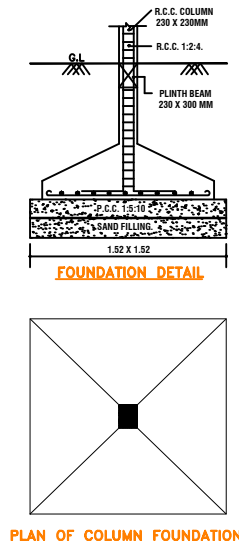
FOUNDATION DETAIL
