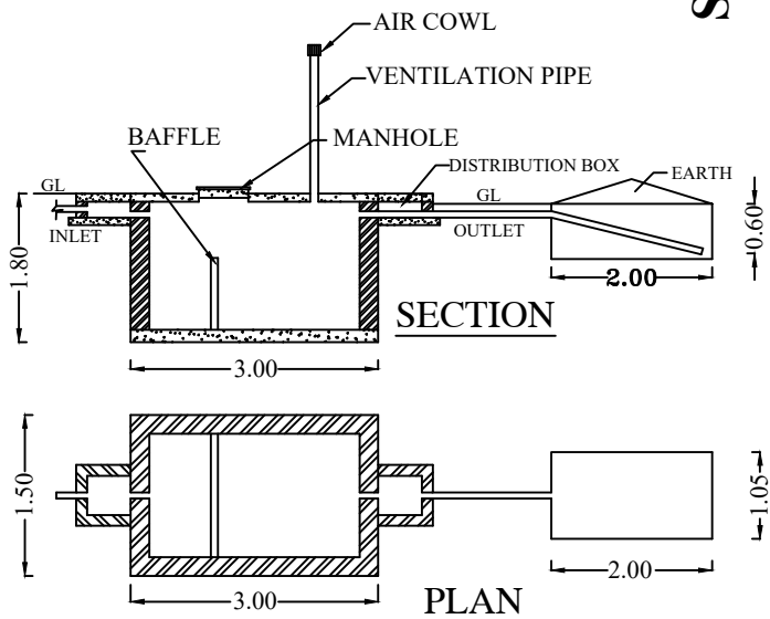
SEPTIC TANK DISPERSION TRENCH
