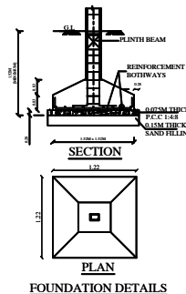
FOUNDATION DETAILS
