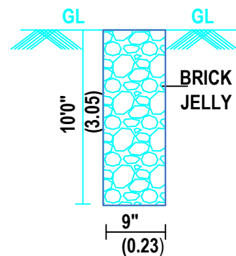
PERCULATION PIT
