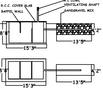
SEPTIC TANK AND DISPERSION TRENCH DETAILS
