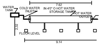
SOLAR HOT WATER SYSTEM DETAILS
