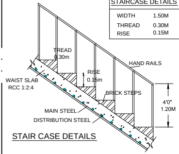
STAIRCASE DETAILS
