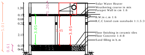
SECTION - "AB "
