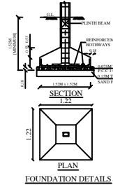
FOUNDATION DETAILS
