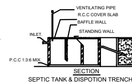
SECTION SEPTIC TANK & DISPOSITION TRENCH
