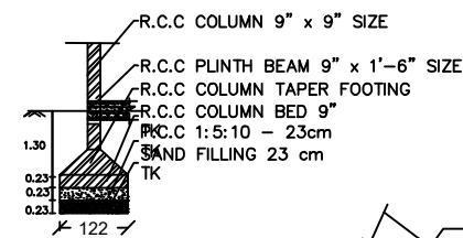
SECTION COLUMN DETAILS PLAN
