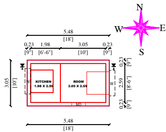
PRO.GROUND FLOOR
