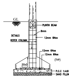
FOUNDATION DETAILS
