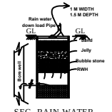
SEC. RAIN WATER HARVEST PIT
