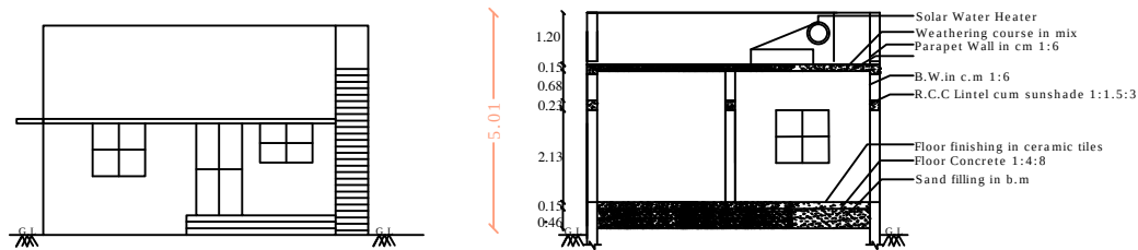
SECTION "AB"
