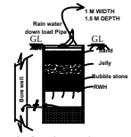
SEC. RAIN WATER HARVEST PIT
