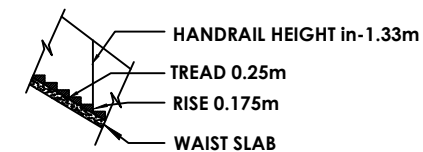
STAIRCASE DETAILS
