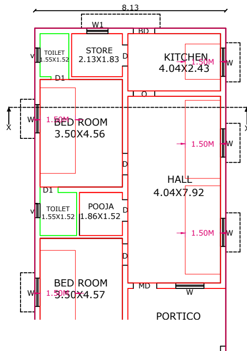
PLAN
