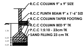
SECTION COLUMN DETAILS PLAN
