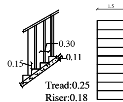
STAIRCASE DETAIL
