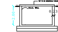
RWH SECTION (SAMPLE)
