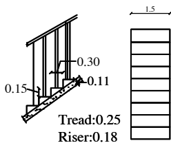
STAIRCASE DETAIL
