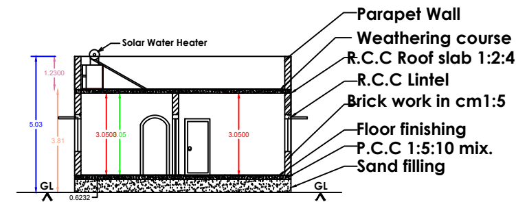
SECTION ON ABCD
