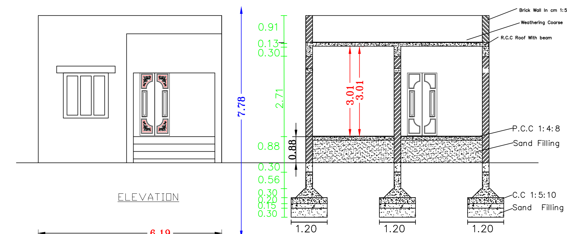
SECTION "AA"
