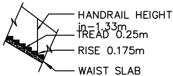
STAIRCASE DETAILS
