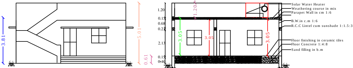
SECTION - "AB "
