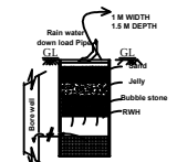
SEC. RAIN WATER HARVEST PIT
