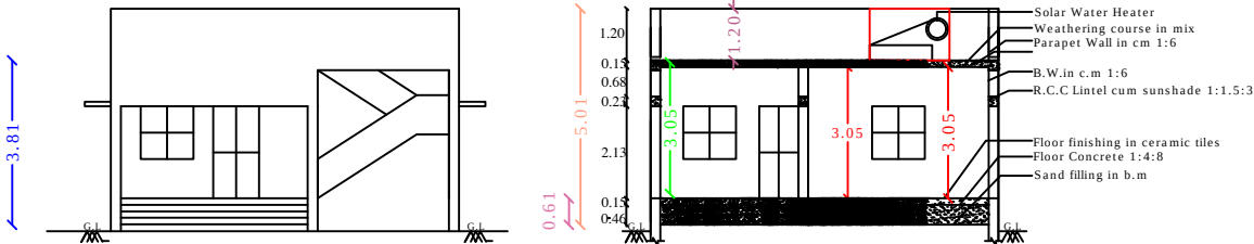
SECTION - "AB "
