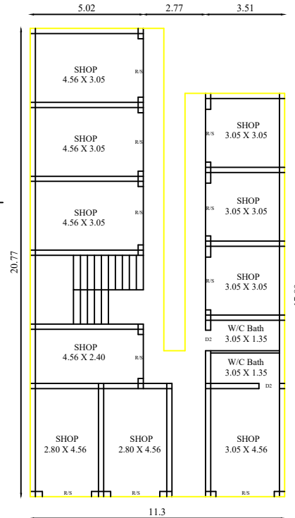
EXIST GROUND FLOOR
