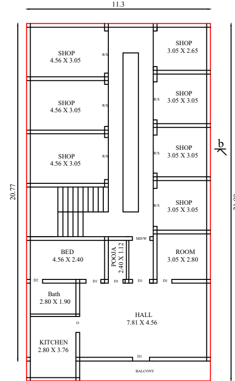
PROP FIRST FLOOR
