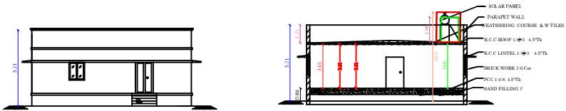
CUT SECTION ON AA
