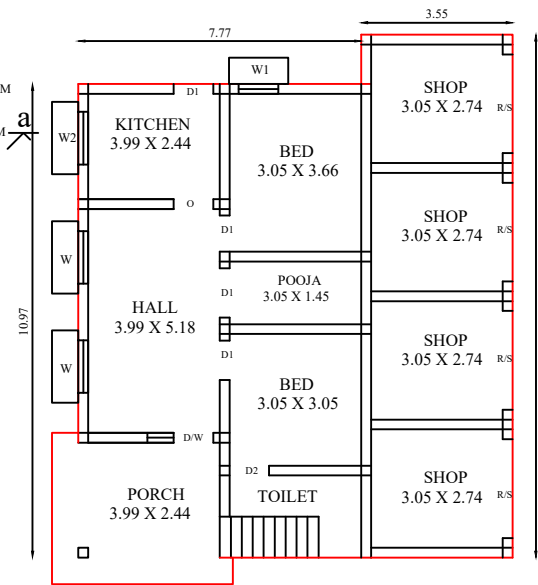
PROPOSED PLAN
