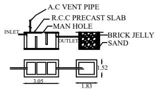
DETAIL DISPE
