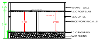
SECTION ON A-A
