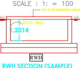
RWH SECTION (SAMPLE)
