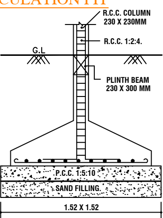
FOUNDATION DETAIL
