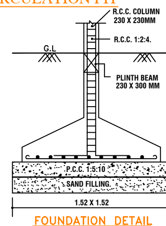
FOUNDATION DETAIL
