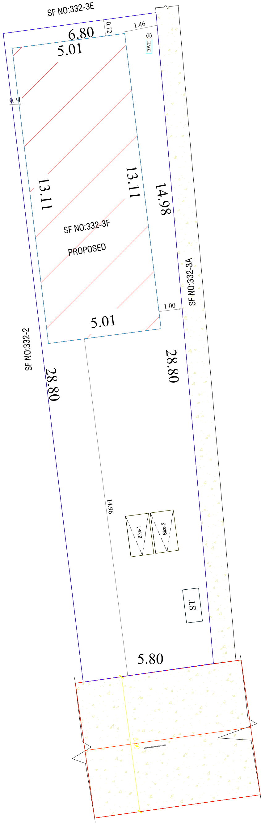
SITE PLAN
