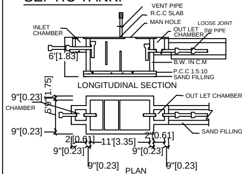
SEPTIC TANK:
