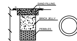
RAIN WATER HARVESTING SYSTEM
