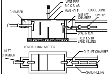
SEPTIC TANK
