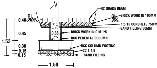
FOUNDATION DETAIL
