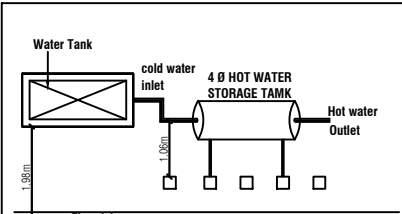
SOLAR HOT WATER SYSTEM (SWHS) DETAIL
