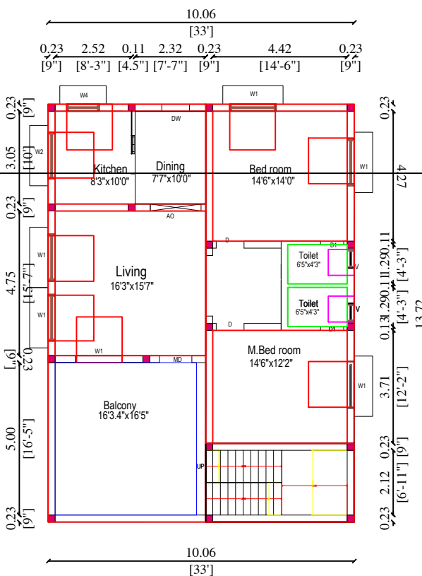
EXISTING & PROPOSED FIRST FLOOR PLAN
