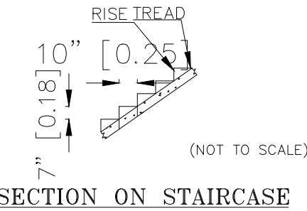
SECTION ON STAIRCASE
