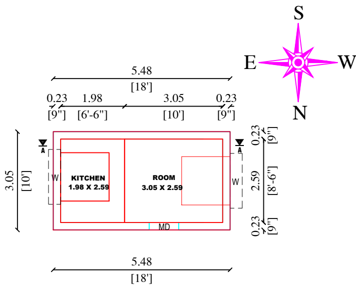
PRO.GROUND FLOOR
