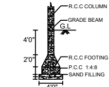
COLOUMN FOUNDATION
