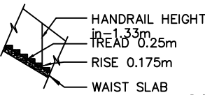
STAIRCASE DETAILS
