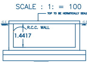
RWH SECTION (SAMPLE)
