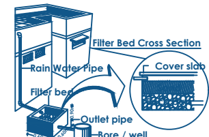
DETAILS OF RWH
