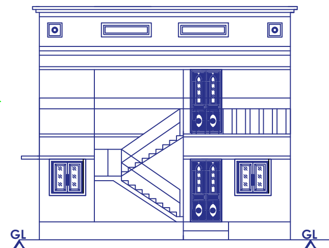
FRONT ELEVATION
