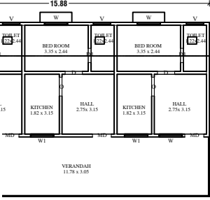
IRST FLOOR PLAN
