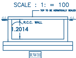
RWH SECTION (SAMPLE)
