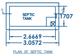
PLAN OF SEPTIC TANK
