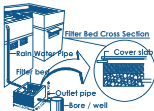
DETAILS OF RWH
